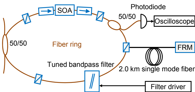
Schematic view of a typical FDML setup
